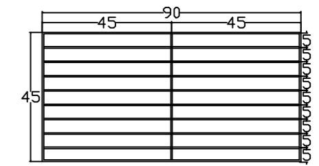
GRADE DE FERRO CHAPA 50X5mm
